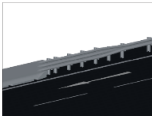
Example of transition from w-beam guardrail to rigid or precast concrete safety barrier using three-beam section
