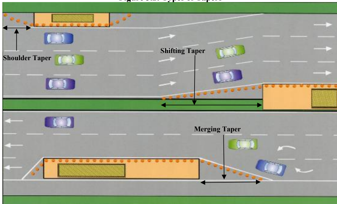
Figure 3.2: Types of Tapers
