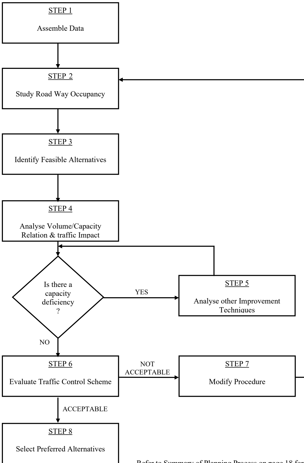
Flowchart 3.1 Planning Flowchart
