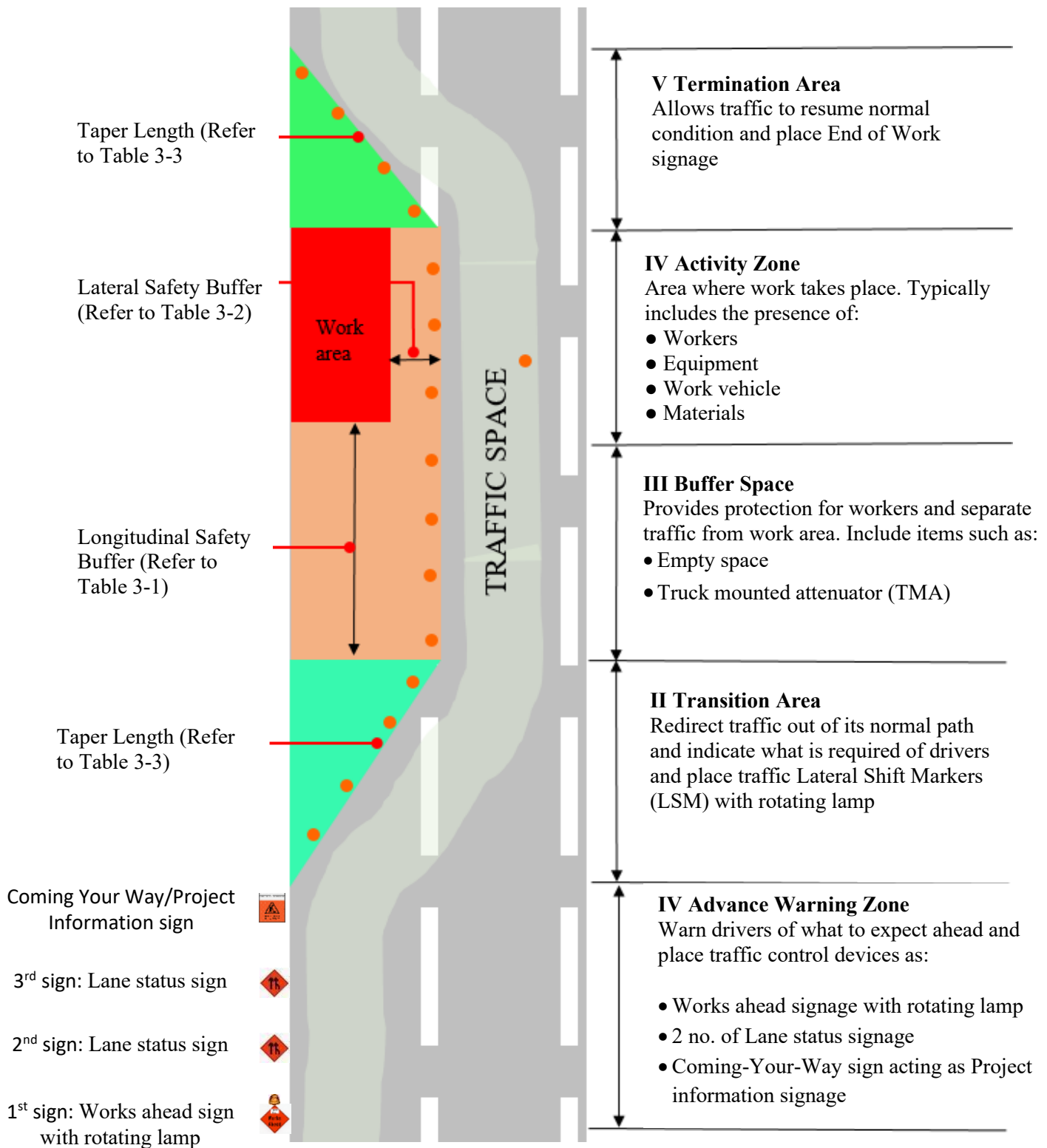
Figure 3.1 Component of an Activity Zone
