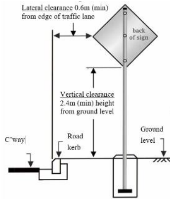
Example of support for post-mounted sign
